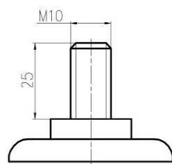
丝杆 Threaded Stem
