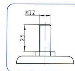
丝扣 threaded stem
