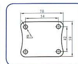
2-2.5寸活动底板 2-2.5" Swivel baseplate
