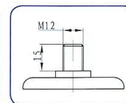
2寸丝扣 2" threaded stem
