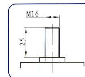
丝扣 Threaded stem
