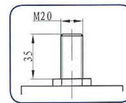
丝扣 Threaded stem
