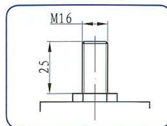
丝扣 Threaded stem
