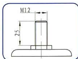
丝扣 Threaded stem
