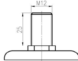
丝杆 Threaded Stem
