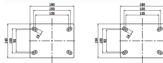
平底活动 Plate of Swivel Caster 固定底板 Plate of Rigid Caster
