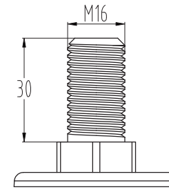
丝杆 Threaded Stem
