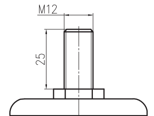
丝杆 Threaded Stem
