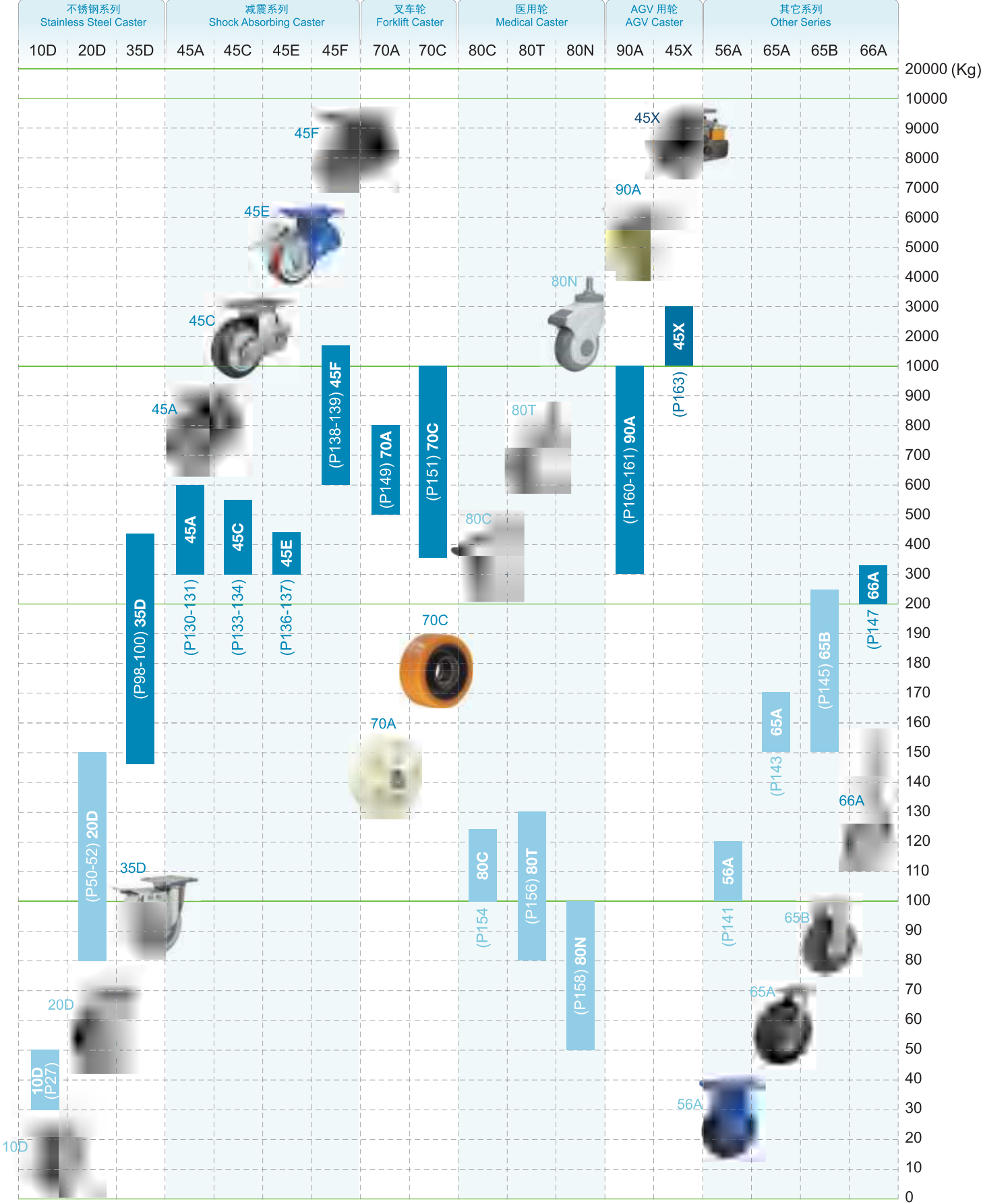
各系列产品载重范围 Capacity Range of Each Series
