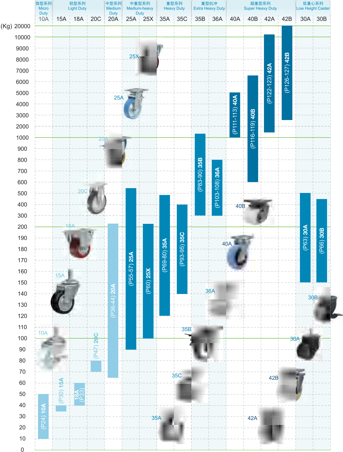
各系列产品载重范围 Capacity Range of Each Series
