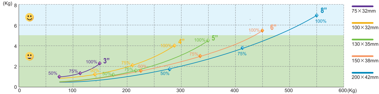
启动阻力 Starting Resistance
