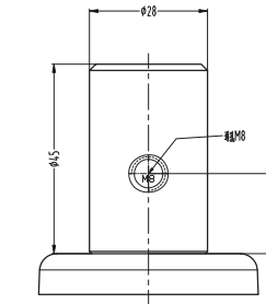
插杆 Stem of Swivel Caster
