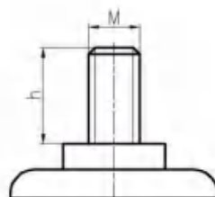
丝杆 Threaded Stem
