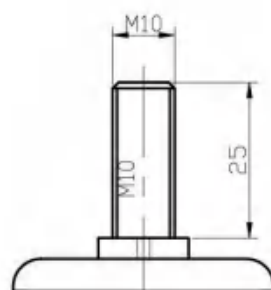
丝杆 Threaded Stem
