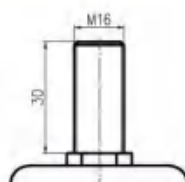
丝杆 Threaded Stem
