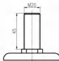
丝杆 Threaded Stem
