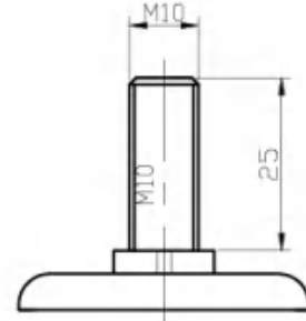
丝杆 Threaded Stem
