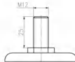
丝杆 Threaded Stem
