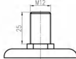
丝杆 Threaded Stem
