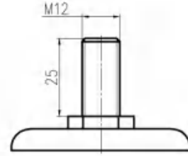
丝杆 Threaded Stem
