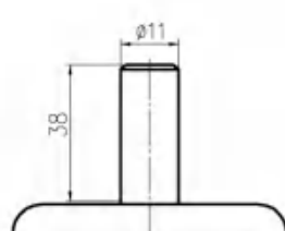
插杆 Stem of Swivel Caster
