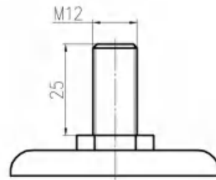
丝杆 Threaded Stem
