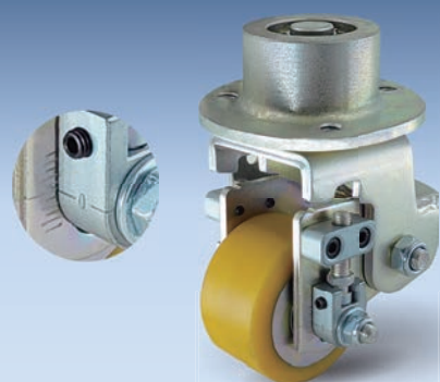
高端叉车平衡轮 Forklift Supporting Caster
