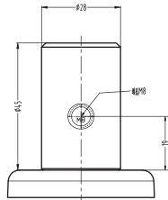
插杆 Stem of Swivel Caster
