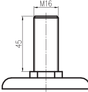
丝杆 Threaded Stem
