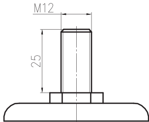
丝杆 Threaded Stem
