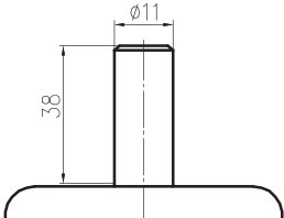
插杆 Stem of Swivel Caster
