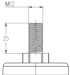
丝杆 Threaded Stem
