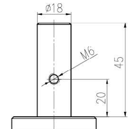
插杆活动/刹车 Stem of Swivel Caster
