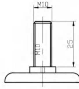
丝杆 Threaded Stem
