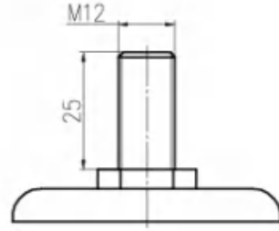
丝杆 Threaded Stem
