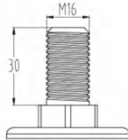
丝杆 Threaded Stem
